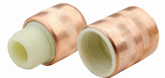
Manguito antielectrólisis MT PN-16 1", 1/2", 3/4". Cobre 99,9%, interior poliamida 6.0 + 30% fibra vidrio. 872F1...
