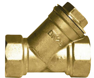
Filtro "Y" tamiz inox MT PN-16 1", 1/2", 3/4". CW617N. Malla inox. 875FY11
